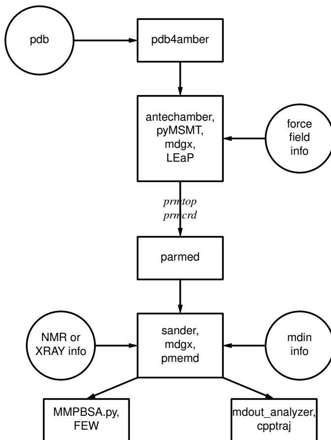
Figure 1.1.: Basic information flow in Amber
