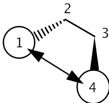
Figure 15.1.: 1-4 Interactions between atoms "1" and "4".
